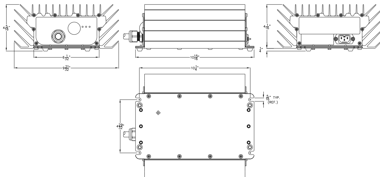
Figure 2-3: Charger Dimensions and Mounting Slot Locations (Case #2)
